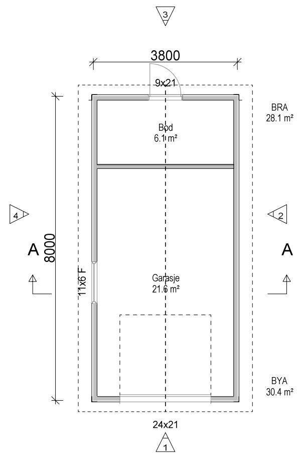
Plan
